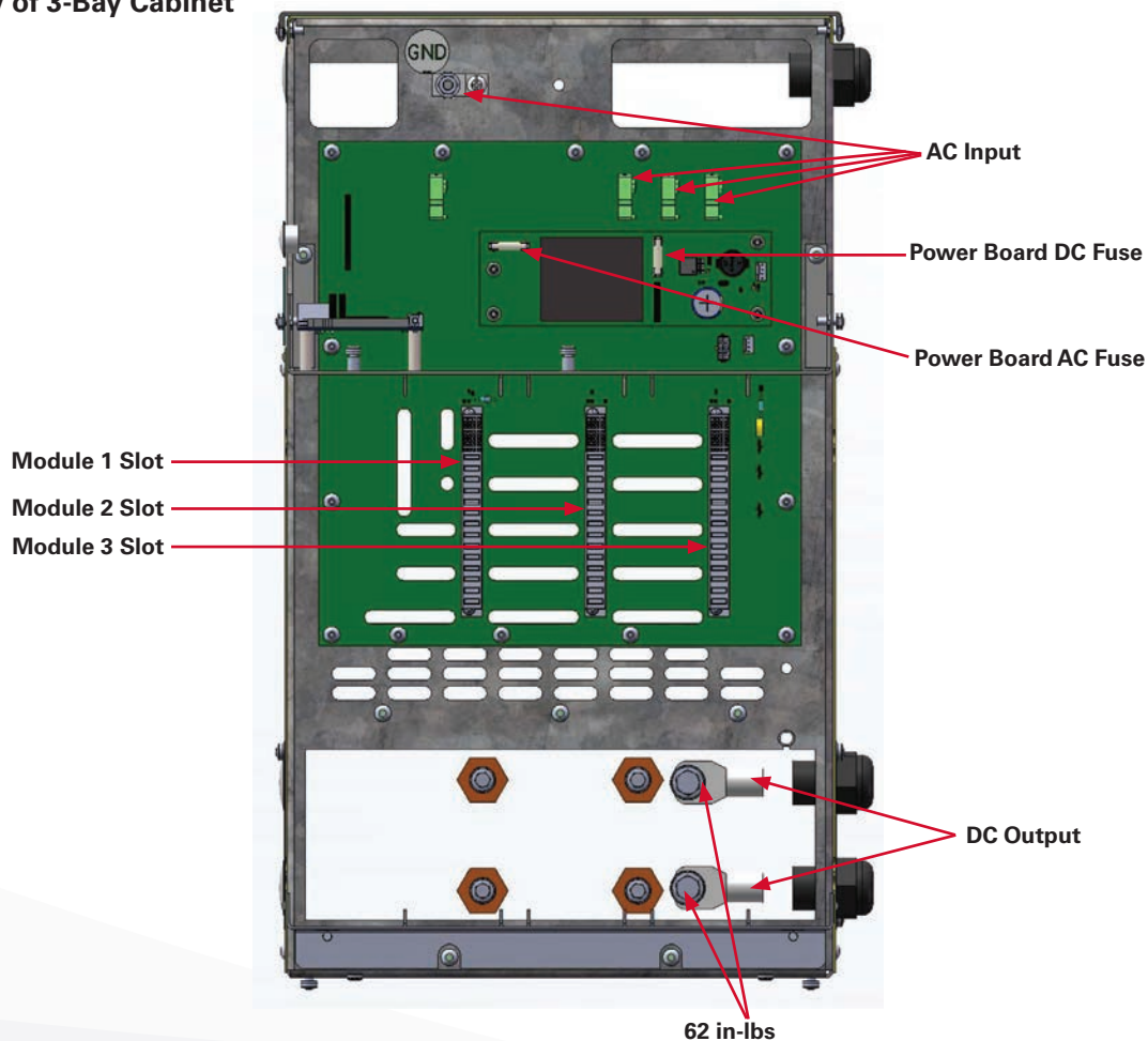
Inside View of 3-Bay Cabinet
